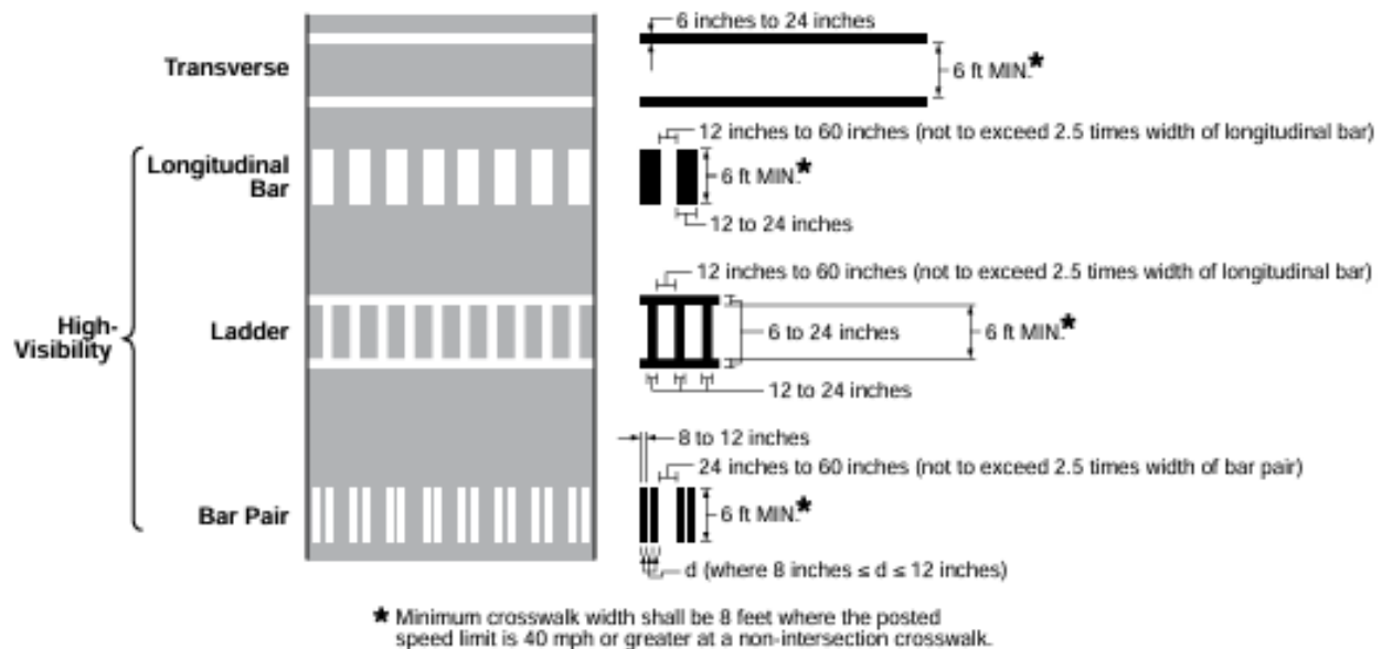
Figure 3C-1. Crosswalk Markings
